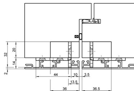
cross section 2
