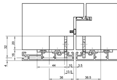
cross section 3
